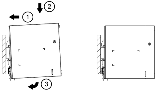
Fig. 3.1 Mounting
